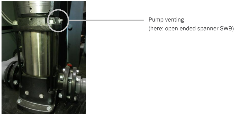
Figure 17: Position of the pump vent (vertical type)
