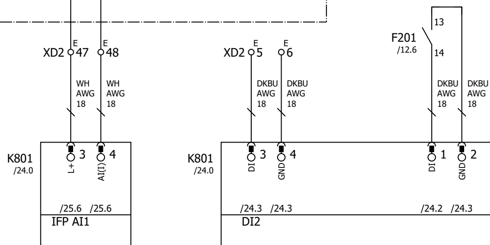
Drucksensor Austritt Pumpe 1 Pressure sensor outlet pump 1
