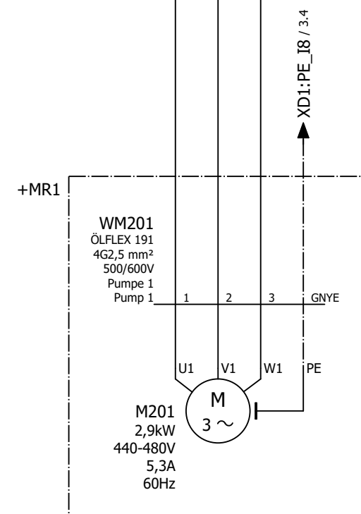
Pumpe 1 Pump 1
