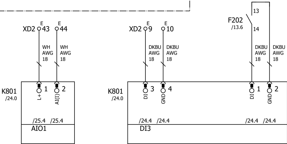
Motorschutzscharter Pumpe 2 Motor overload switch pump 2
